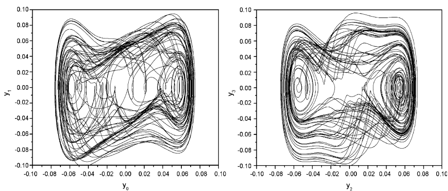
Fig. 10. Hyperchaos: \delta_1 = 0.06 , \delta_2 = 0 and (\theta_1, \theta_2, \theta_3) = (0.7, 1.5, 0.7) .
